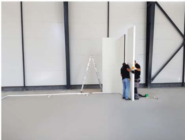
The panels are being installed on the base frame. The panels have interlocking system and are self-standing.
